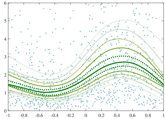
Fig. 2. Regression results by (10) for the quantiles in Fig. 1.
